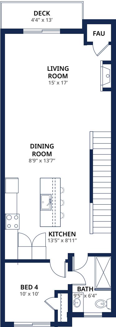
MAIN LEVEL
